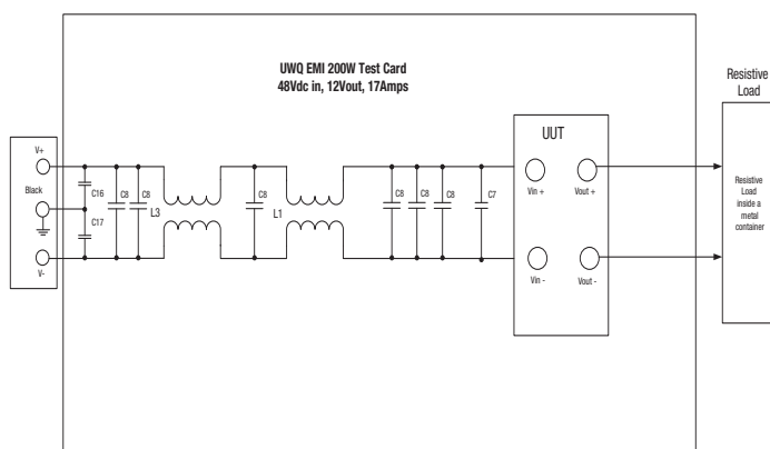
Figure 8. Conducted Emissions Test Circuit
