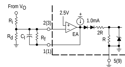
Figure 31. Error Amplifier Compensation
