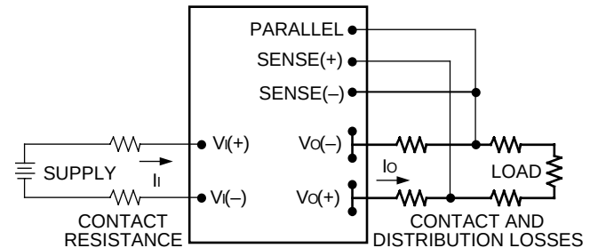
Figure 3. Effective Circuit Configuration for Single-Module Remote Sense Operation
