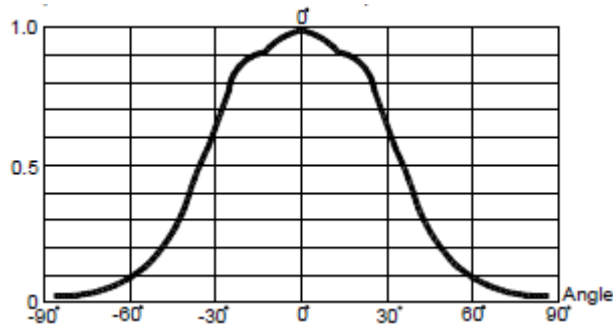
Angular Distribution
