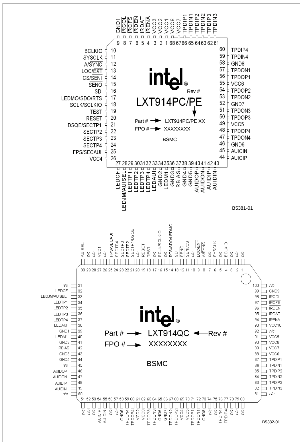
Figure 2. Pin Assignments
