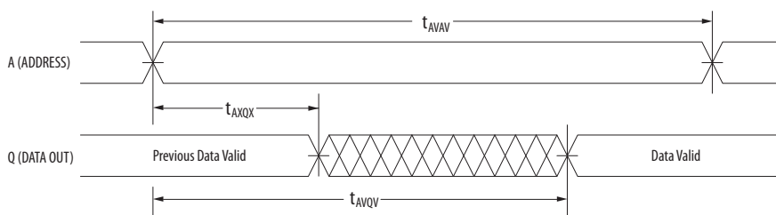
Figure 6 – Read Cycle 1
