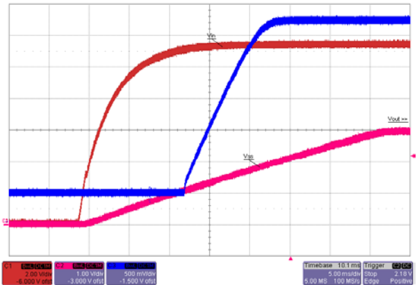
Fig. 8: Pre-Bias Start up, 0A Load Ch_1:V_{in} , Ch_2:V_{SS} , Ch_3:V_{out}
