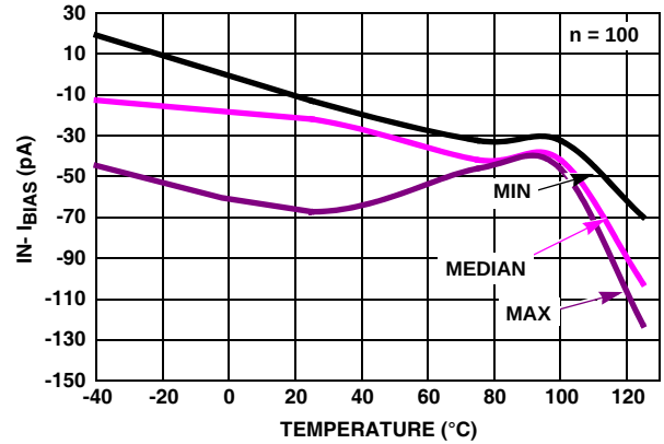
FIGURE 38. I_{BIAS} (IN-) vs TEMPERATURE, V_+ = +5V , V_- = GND
