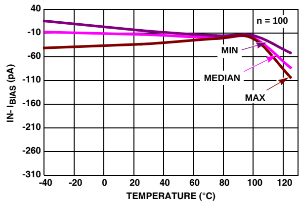
FIGURE 40. I_{BIAS} (IN-) vs TEMPERATURE, V_+ = +1.2V , V_- = GND
