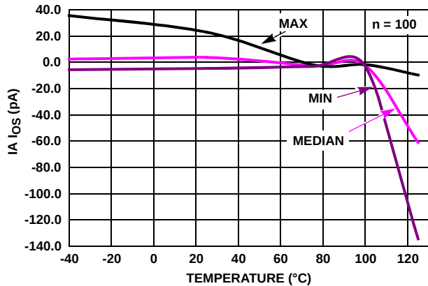
FIGURE 41. I_A INPUT OFFSET CURRENT vs TEMPERATURE, V_+ = +5V , V_- = GND
