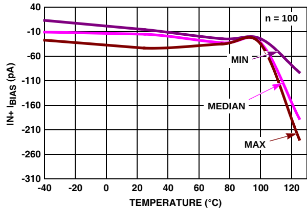
FIGURE 39. I_{BIAS} (IN+) vs TEMPERATURE, V_+ = +1.2V , V_- = GND
