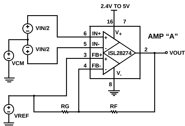
FIGURE 63. REFERENCE CONNECTION WITH AN AVAILABLE V_{REF}
