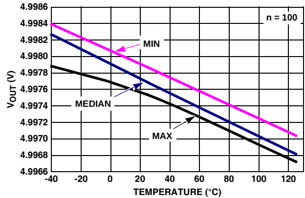
FIGURE 58. V_{OUT} HIGH vs TEMPERATURE, R_L = 100k , V_+ , V_- = \pm 2.5V
