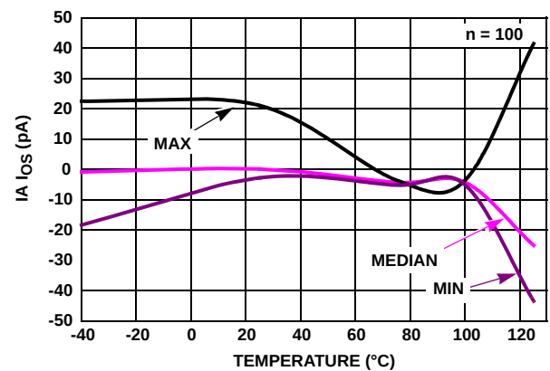
FIGURE 42. I_A INPUT OFFSET CURRENT vs TEMPERATURE, V_+ = +1.2V , V_- = GND
