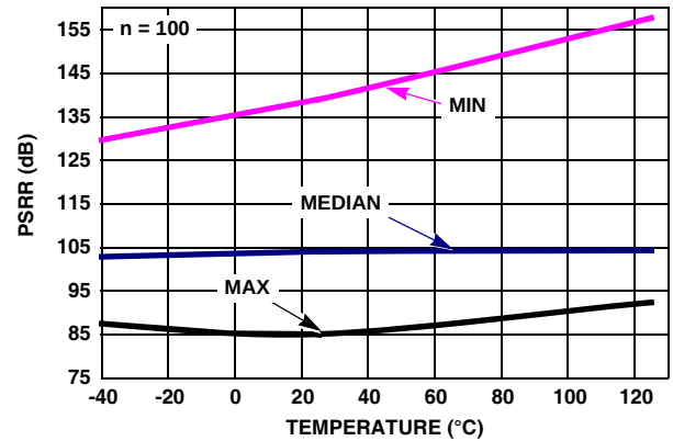
FIGURE 52. PSRR vs TEMPERATURE, V_+ , V_- = \pm 2.5V
