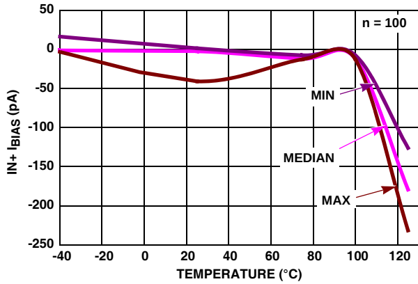
FIGURE 37. I_{BIAS} (IN+) vs TEMPERATURE, V_+ = +5V , V_- = GND
