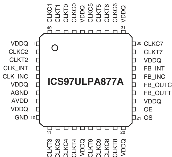
40-Pin MLF
