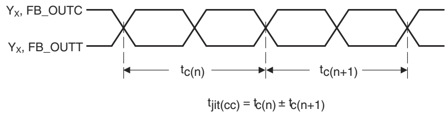
Figure 3. Cycle-to-Cycle Jitter
