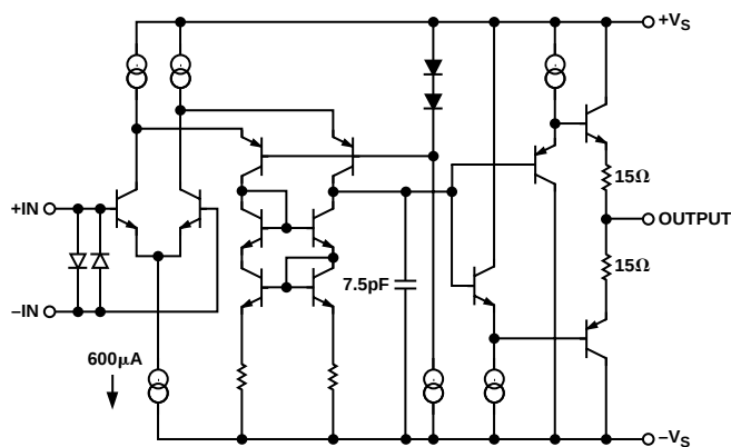
Figure 3. Simplified Schematic
