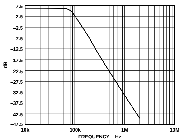
Figure 7. Frequency Response of Sallen-Key Filter
