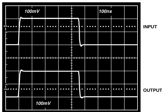
TPC 9. Noninverting Small Signal Pulse Response, R_L = 500 \Omega , V_S = \pm 12 \text{ V} , G = +1 , R_F = 0
