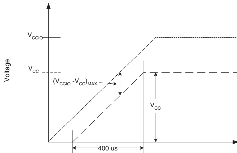
Figure 30: Power-up Sequencing
