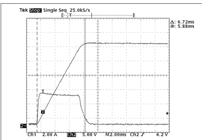
Figure 4 – Inrush Limiting: Inrush current with 1000 μF external capacitance.
