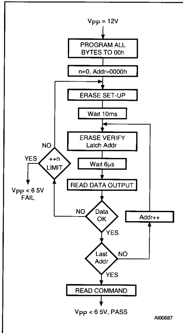
Figure 12. Erasing Flowchart
