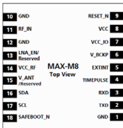
Figure 2: Pin Assignment
