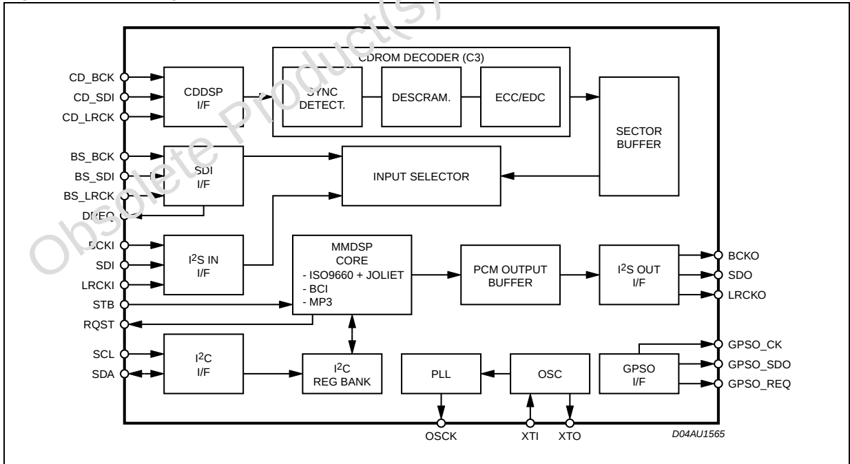
Figure 3. Block Diagram
