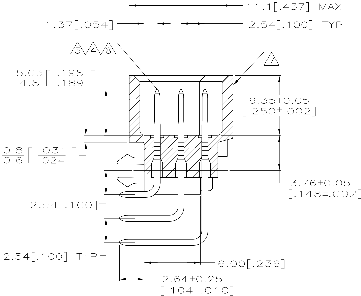
SECTION X-X
