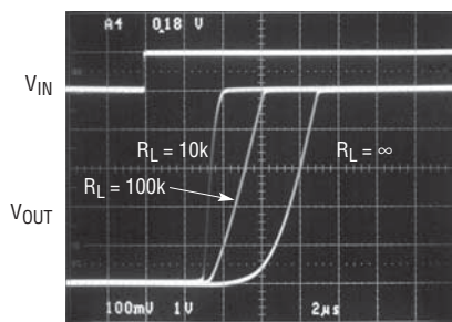
LT1018 Response Time
