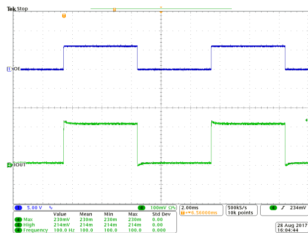
Figure 6: V_{OUT} Sink Current. OE Pin 6V Square Wave, I_{SET} = 3\text{k}\Omega , V_{DROP} = 0.5\text{V}
