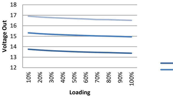
AM1/4S-0515SZ Load vs. Vout
