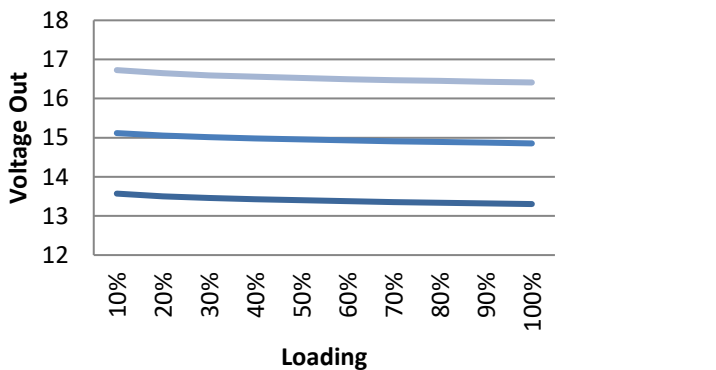
AM1/4S-1215SZ Load vs. Vout
