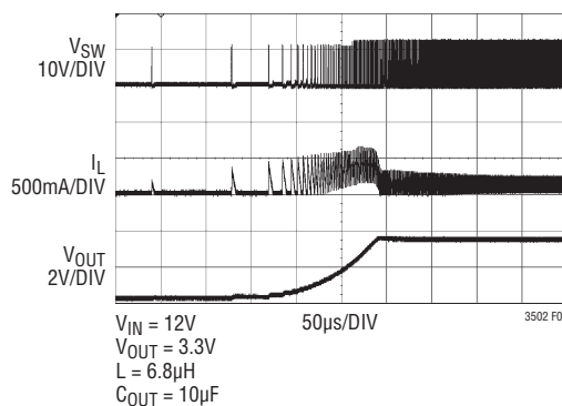
Figure 7. To Soft-Start the LT3502A, Add a Resistor and Capacitor to the \overline{\text{SHDN}} Pin
