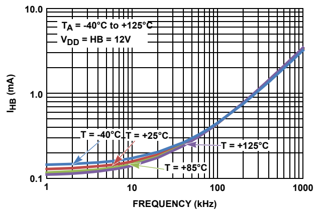
FIGURE 6. I_{HB} OPERATING CURRENT vs FREQUENCY, R_{DT} = 47\text{k}\Omega
