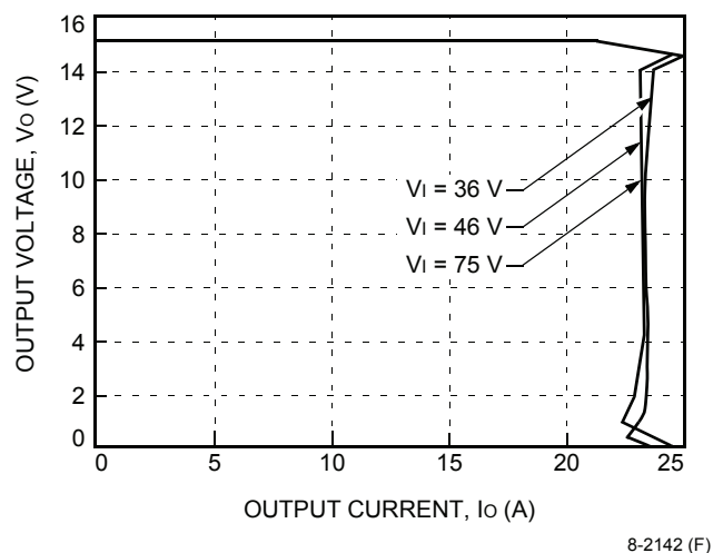
Figure 2. Typical FW300C1 Output Characteristics at Room Temperature
