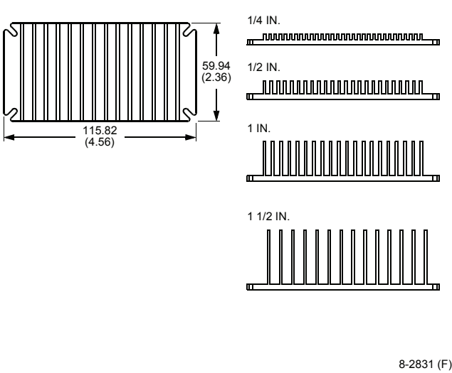
Figure 26. Transverse Heat Sink
