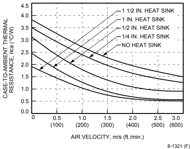
Figure 21. Case-to-Ambient Thermal Resistance Curves; Transverse Orientation
