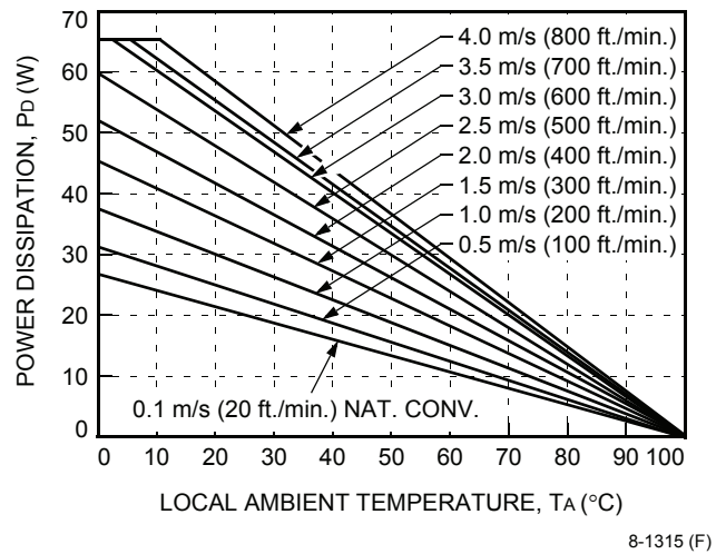
Figure 19. Convection Power Derating with No Heat Sink; Airflow Along Width (Transverse)
