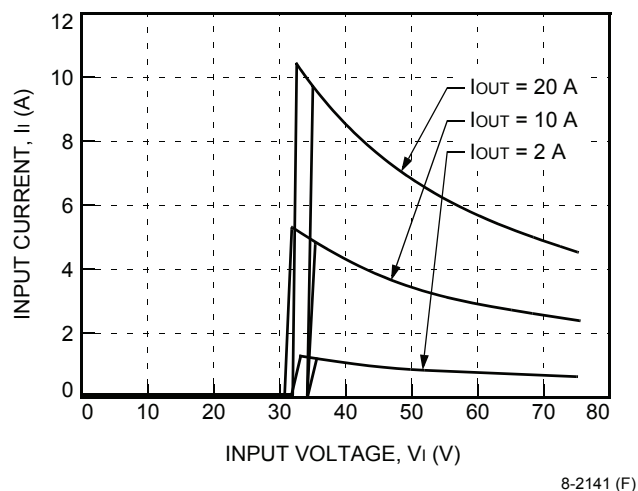
Figure 1. Typical FW300C1 Input Characteristics at Room Temperature, I_o = Full Load
