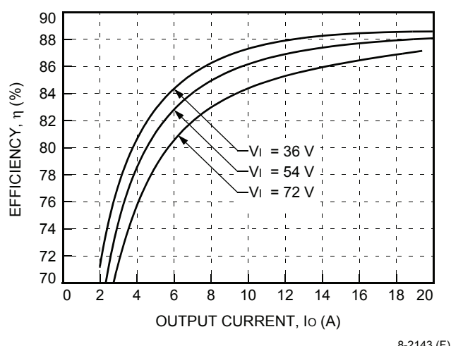
Figure 3. Typical FW300C1 Efficiency vs. Output Current at Room Temperature
