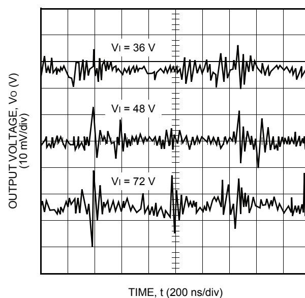
Figure 4. Typical FW300C1 Output Ripple Voltage at Room Temperature and 20 A Output
