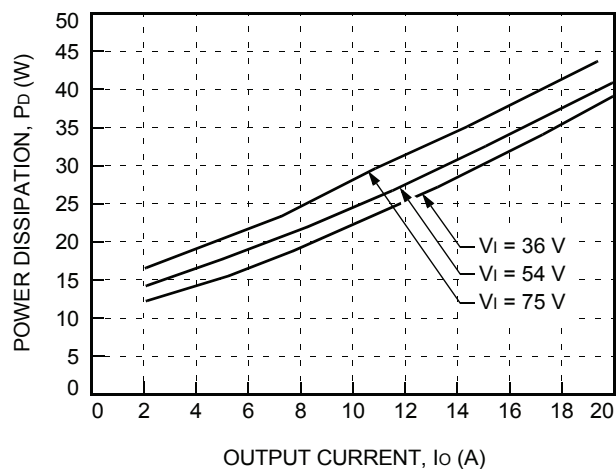
Figure 23. FW300C1 Power Dissipation vs. Output Current at 25 °C
