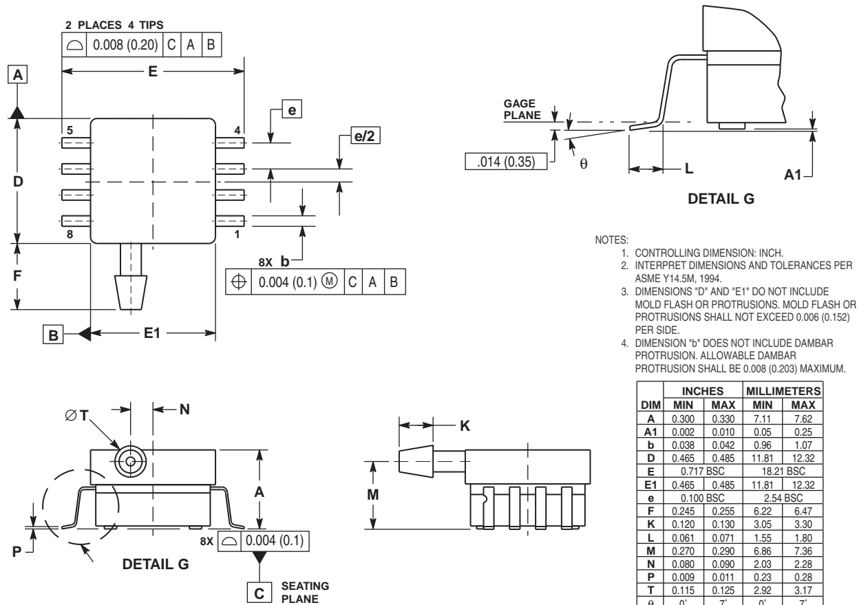
CASE 1369-01 ISSUE O SMALL OUTLINE PACKAGE
