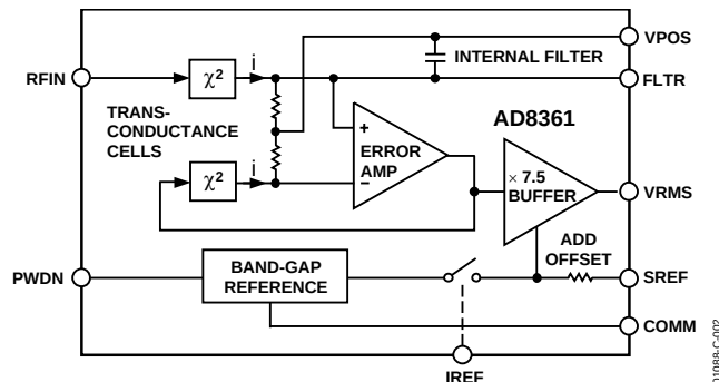
Figure 2. 8-Lead MSOP
