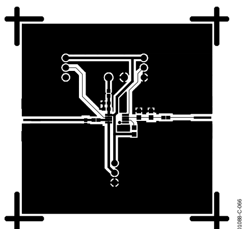
Figure 61. Layout of Component Side, MSOP
