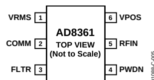
Figure 5. 6-Lead SOT-23
