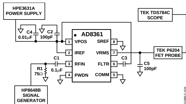
Figure 26. Hardware Configuration for Output Response to Modulated Pulse Input
