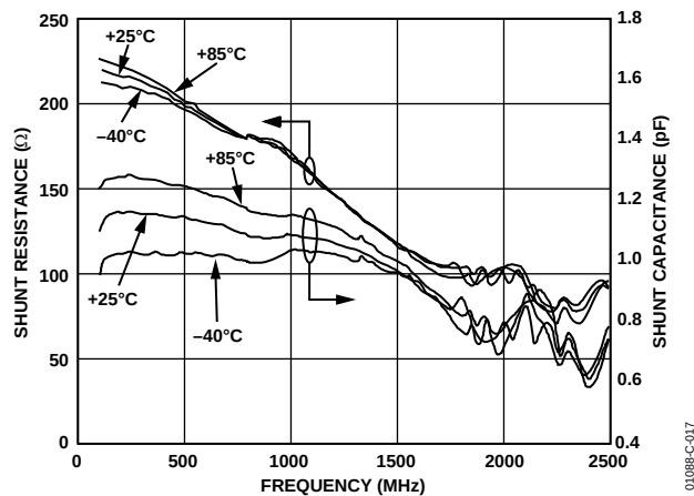
Figure 17. Input Impedance vs. Frequency, Supply 3 V, Temperatures -40°C, +25°C, and +85°C, MSOP (See the Application Information Section for SOT-23 Data)
