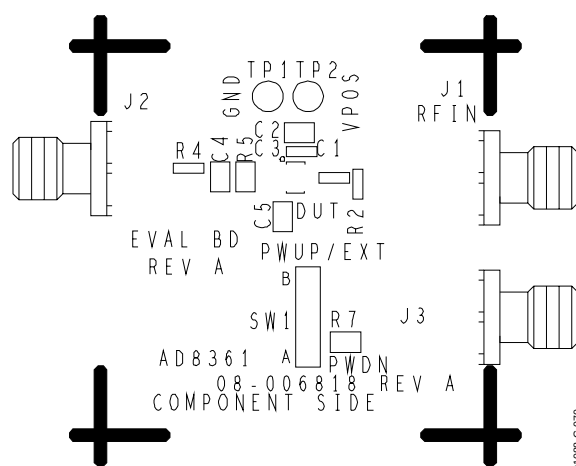
Figure 65. Silkscreen of the Component Side, SOT-23
