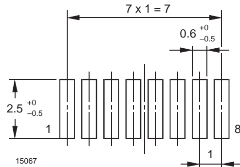
Figure 8. TFDU4100 BabyFace (Universal)
