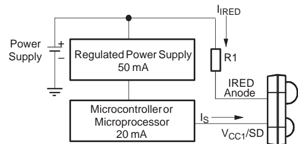
TFDU4100 (Note: Typical Values Listed)
