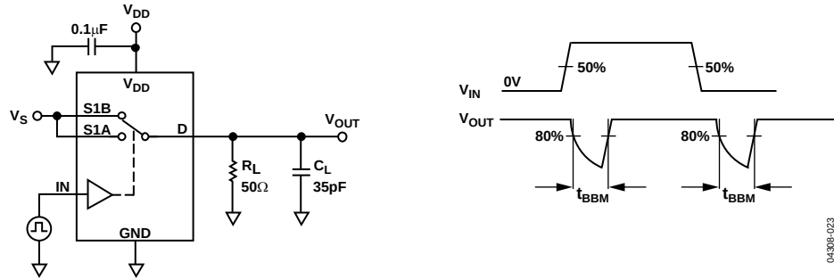
Figure 23. Break-Before-Make Time Delay, t_{BBM}
