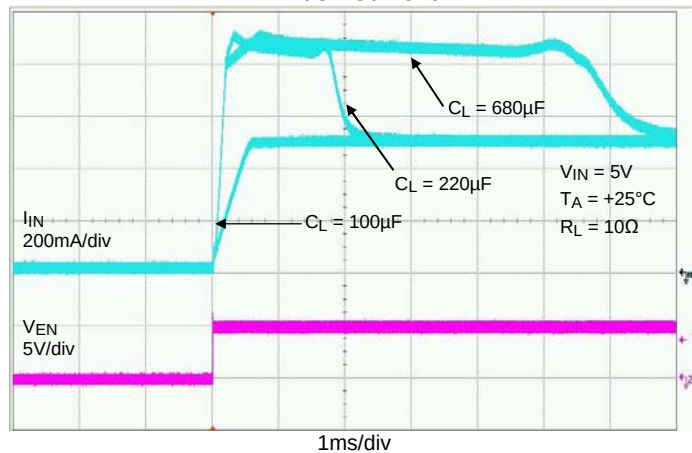
Inrush Current
