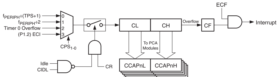
Figure 15-1. PCA Timer/Counter
