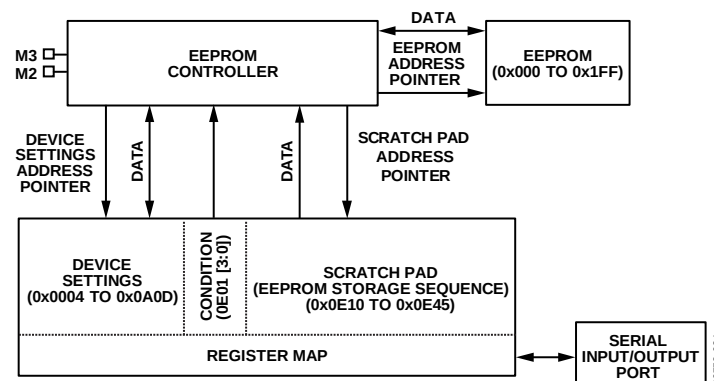
Figure 44. EEPROM Functional Diagram
