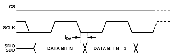
Figure 49. Timing Diagram for Serial Control Port Register Read
