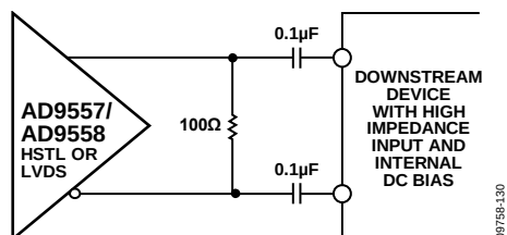
Figure 30. AC-Coupled LVDS or HSTL Output Driver (100 \Omega resistor can go on either side of decoupling capacitors and should be as close as possible to the destination receiver.)
