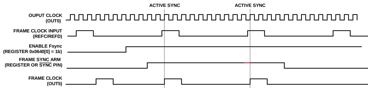
Figure 41. Frame Synchronization in Level Sensitive Mode
