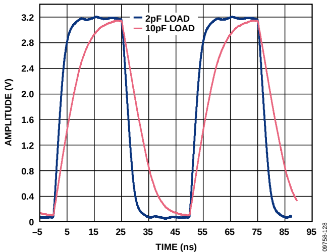
Figure 27. Output Waveform, 3.3 V CMOS (20 MHz, Weak Mode)
