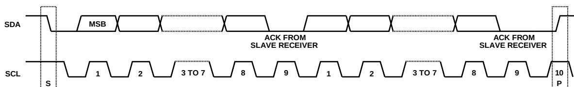
Figure 54. Acknowledge Bit
