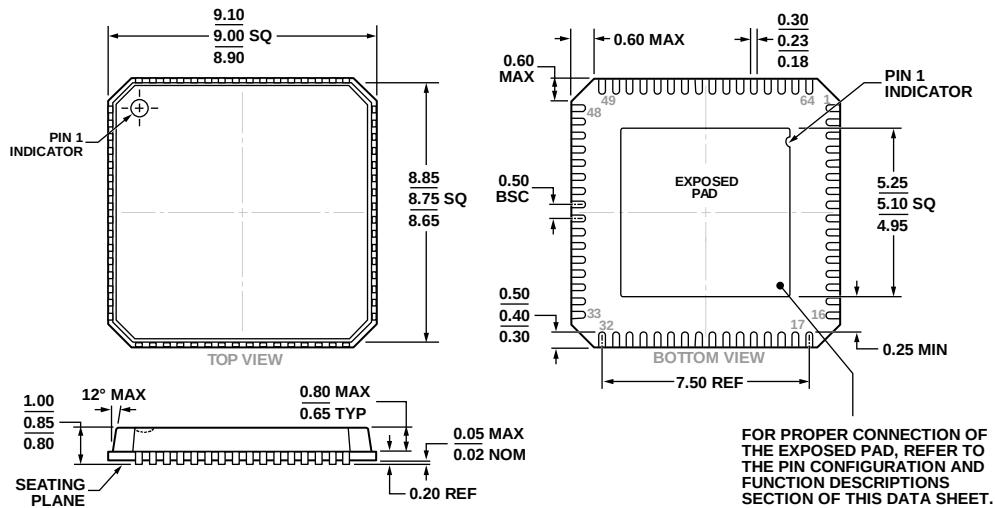
Figure 58. 64-Lead Lead Frame Chip Scale Package [LFCSP_VQ] 9 mm × 9 mm Body, Very Thin Quad (CP-64-5)
