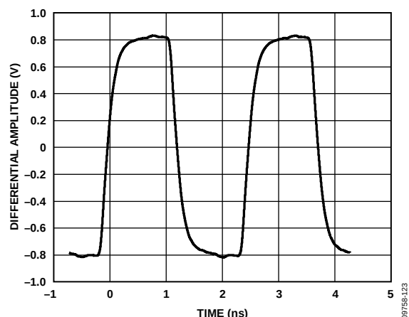
Figure 23. Output Waveform, HSTL (400 MHz)
