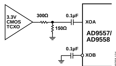
Figure 34. System Clock Input (XOA, XOB) When Using a TCXO/OCXO with 3.3 V CMOS Output
