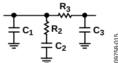
Figure 37. Third Order Analog Loop Filter
