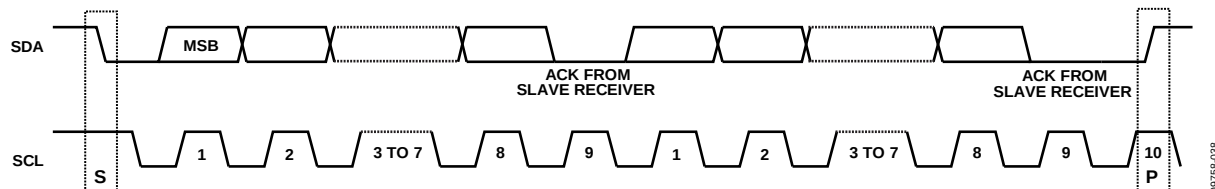
Figure 55. Data Transfer Process (Master Write Mode, 2-Byte Transfer)
