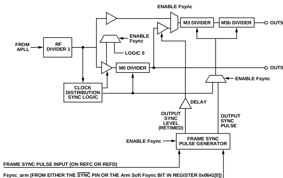
Figure 42. Frame Synchronization in One Shot Mode
