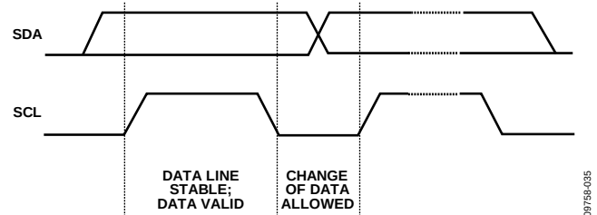
Figure 52. Valid Bit Transfer
