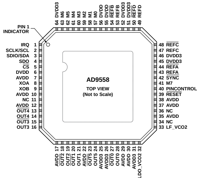
Figure 2. Pin Configuration
