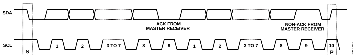
Figure 56. Data Transfer Process (Master Read Mode, 2-Byte Transfer)
