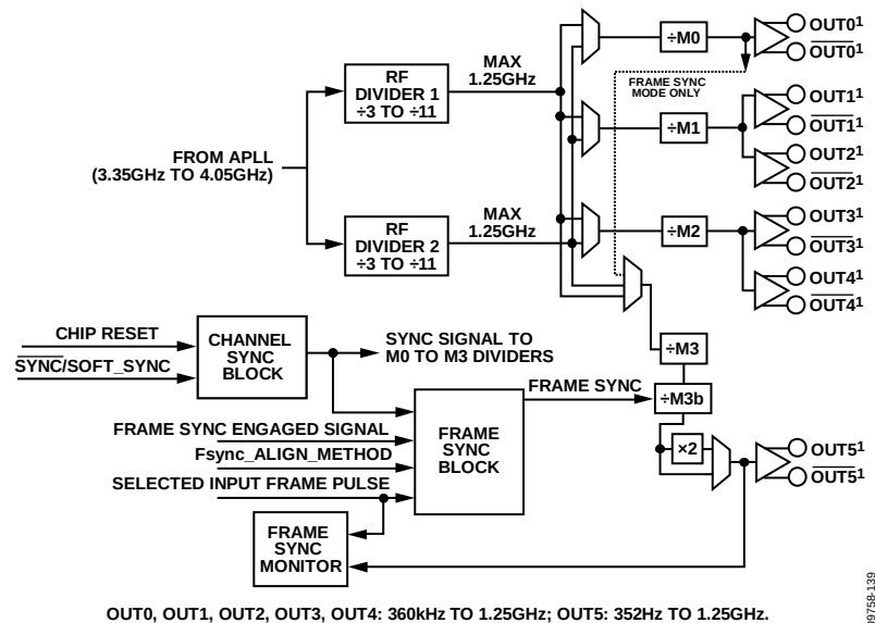
Figure 40. Clock Distribution Block Diagram
