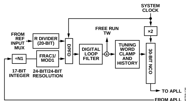
Figure 36. Digital PLL Core
