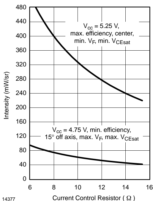
Figure 4. le vs. R1
