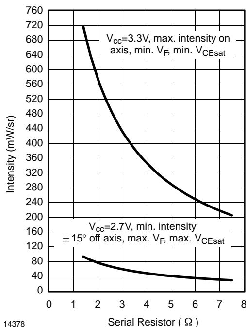
Figure 5. le vs. R1
