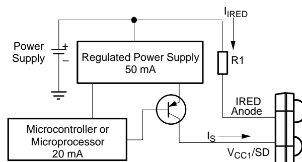
TFDU4100 (Note: Typical Values Listed) Receive Mode @ 5 V: I_{IRED} = 210 mA, I_S = 1.3 mA @ 2.7 V: I_{IRED} = 210 mA, I_S = 1.0 mA Transmit Mode @ 5 V: I_{IRED} = 210 mA, I_S = 5 mA (Avg.) @ 2.7 V: I_{IRED} = 210 mA, I_S = 3.5 mA (Avg.) 14879
