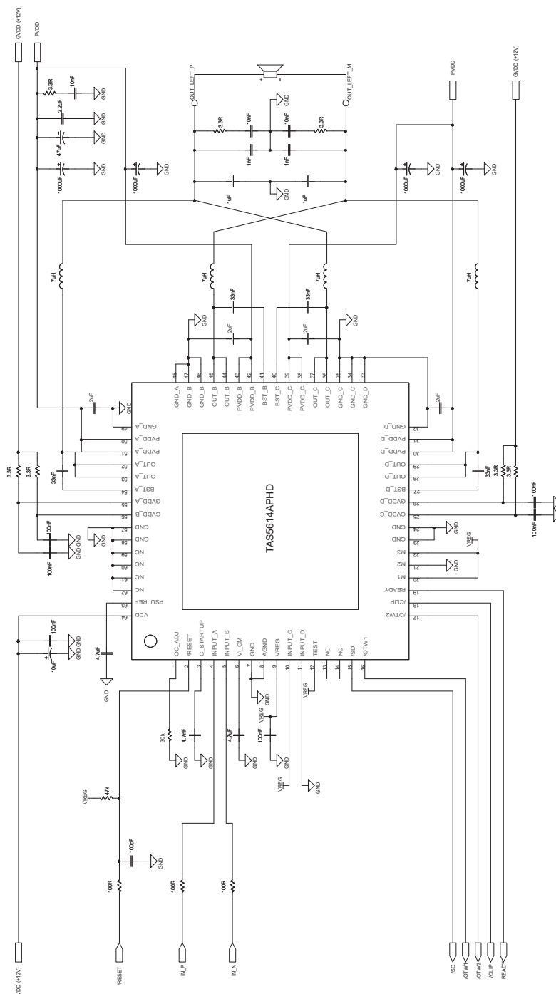
Figure 13. Typical (2N) PBT Application With BD Modulation Filters
