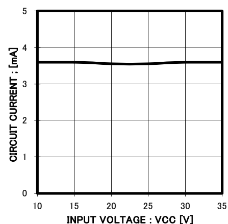
Fig.15 CIRCUIT CURRENT- INPUT VOLTAGE NO LOAD
