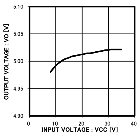
Fig.14 OUTPUT VOLTAGE-INPUT VOLTAGE (Vo=5V, Ro=50hm)
