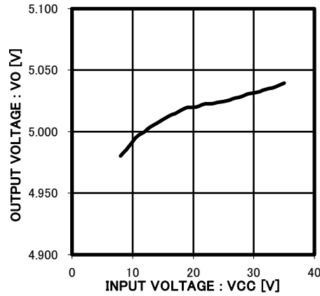
Fig.5 OUTPUT VOLTAGE-INPUT VOLTAGE (Vo=5V, Ro=50hm)
