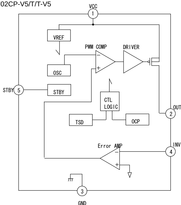
Fig.28 Block Diagram
