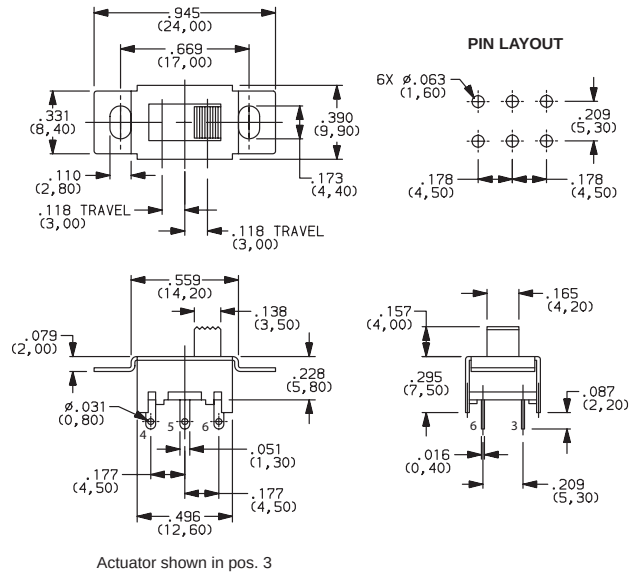
OS203013MT7QN1 DP3T
