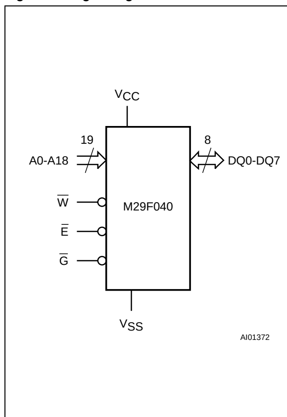
Figure 1. Logic Diagram
