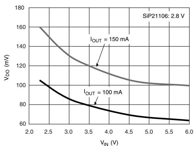
Dropout Voltage vs. Input Voltage
