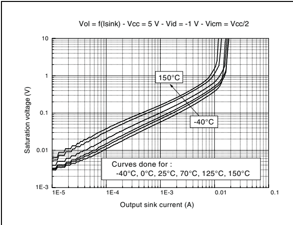
Figure 5. Output saturation voltage vs. output current ( V_{CC} = 5\text{ V} )
