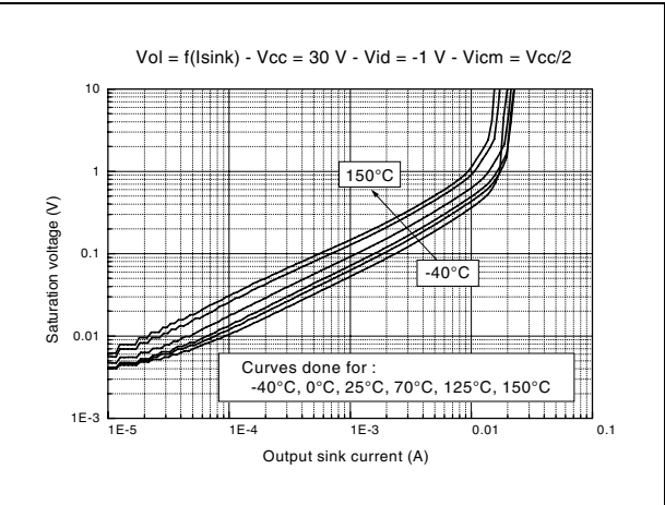
Figure 6. Output saturation voltage vs. output current ( V_{CC} = 30\text{ V} )
