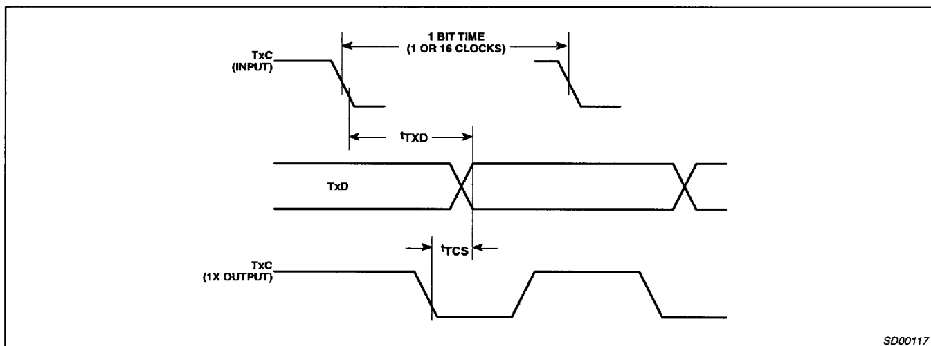
Figure 9. Transmit Timing
