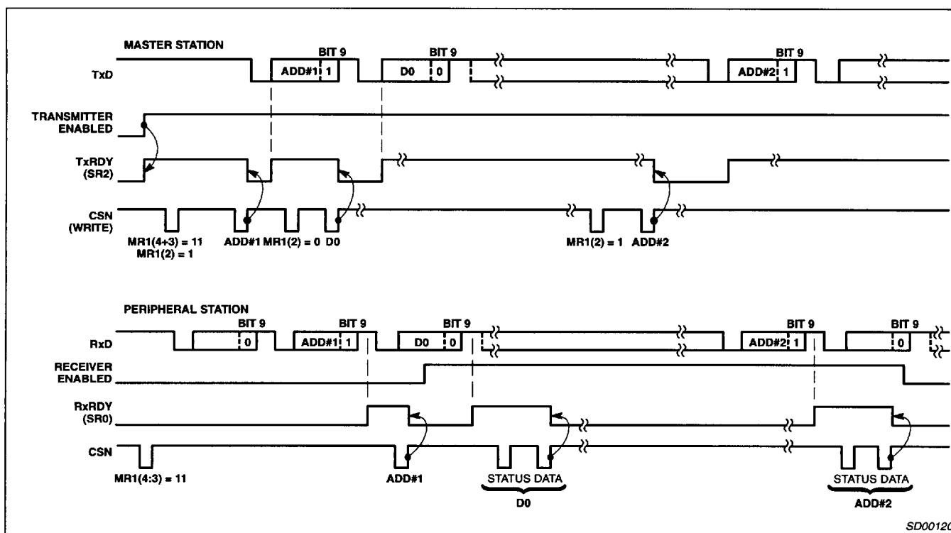
Figure 13. Wake-Up Mode
