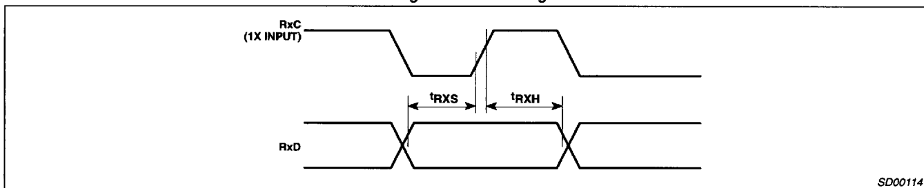
Figure 6. Receive Timing
