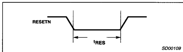
Figure 1. Reset Timing
