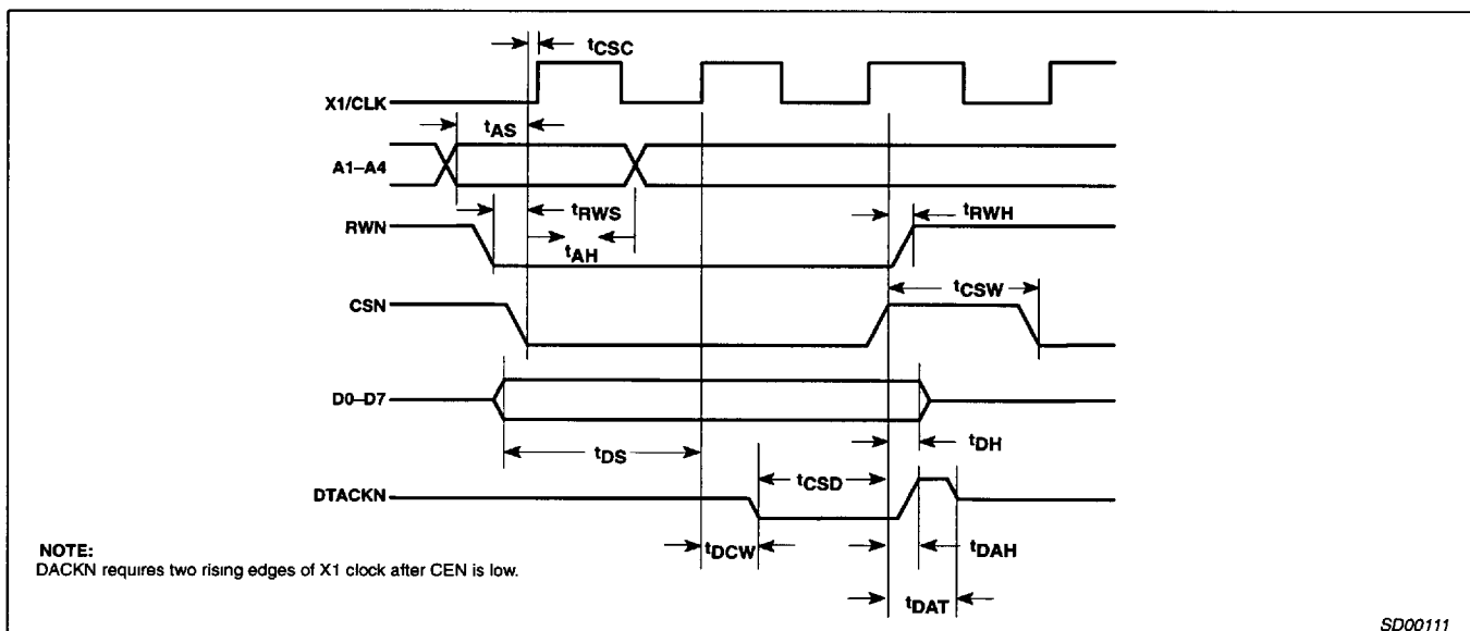
Figure 3. Bus Timing (Write Cycle)
