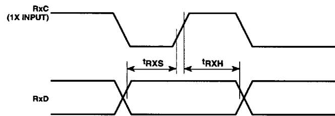
Figure 10. Receive Timing
