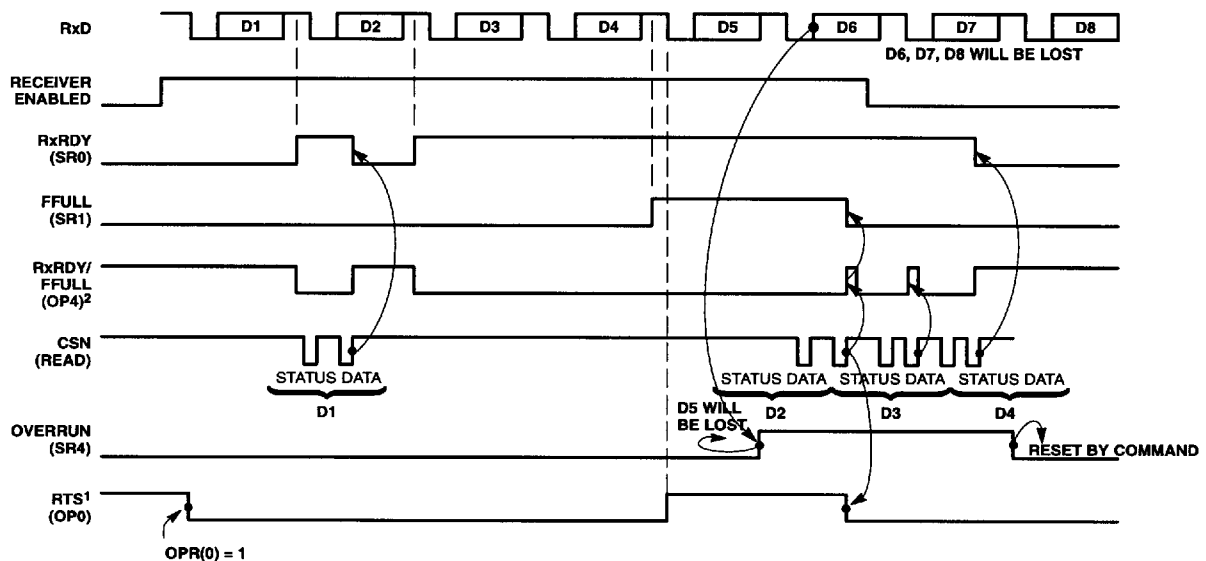
Figure 11. Transmitter Timing
