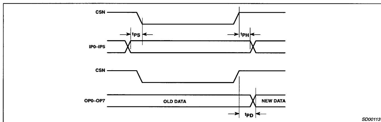
Figure 5. Port Timing
