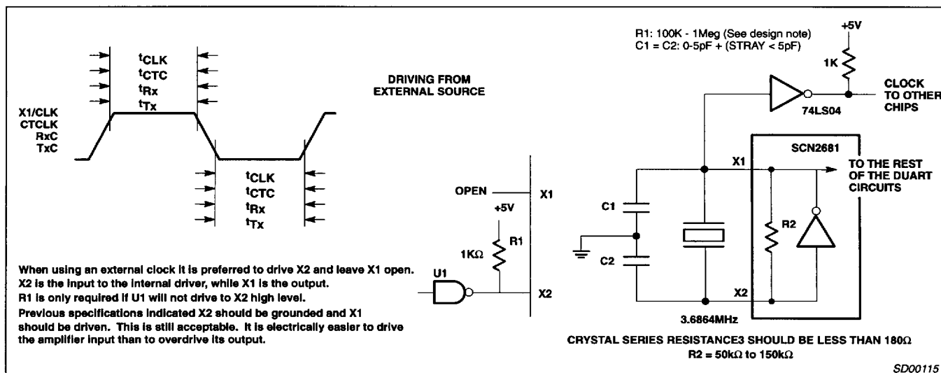
Figure 7. Clock Timing
