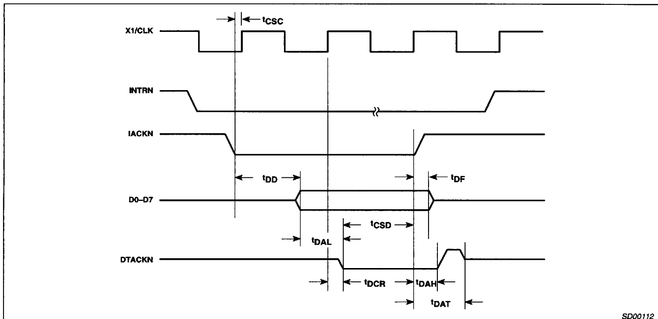
Figure 4. Interrupt Cycle Timing
