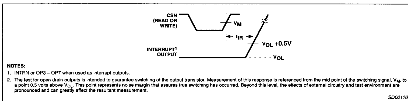
Figure 8. Interrupt Timing
