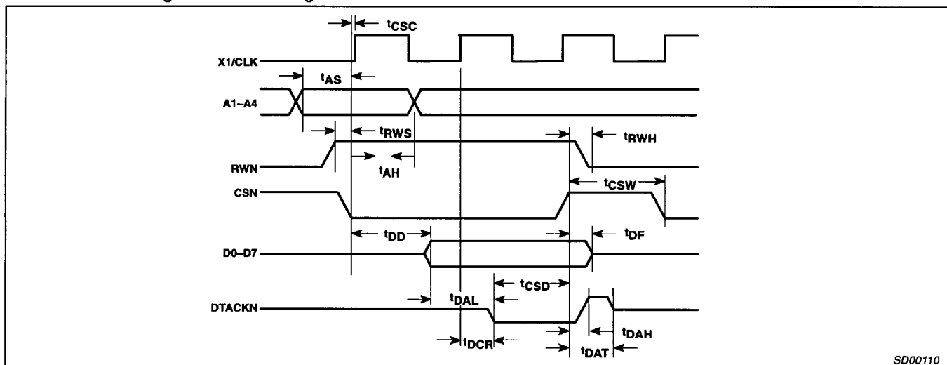
Figure 2. Bus Timing (Read Cycle)
