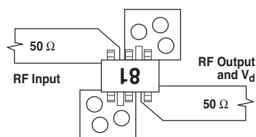
Figure 13. RF Layout.
