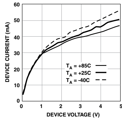
Figure 8. Device Current vs. Voltage and Temperature.
