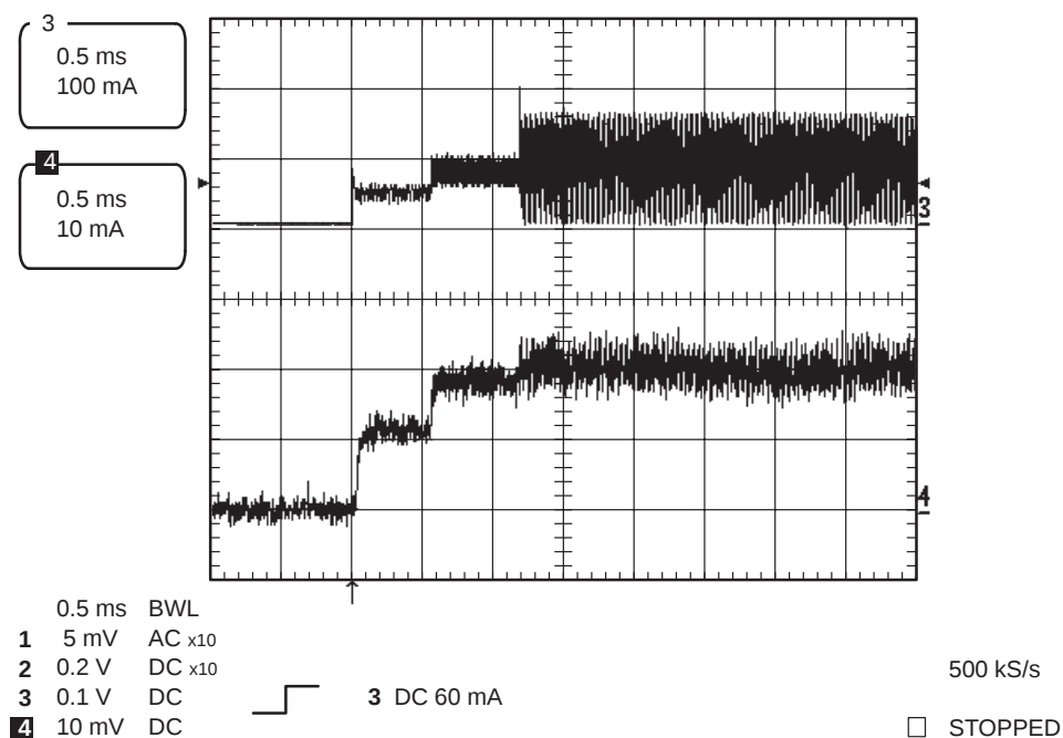
Figure 2–1. Start-up Waveforms
