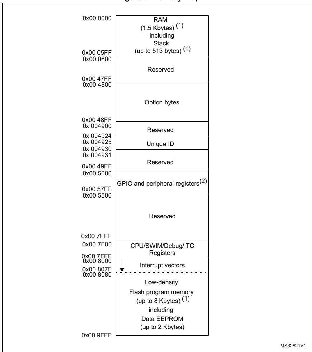
Figure 8. Memory map
