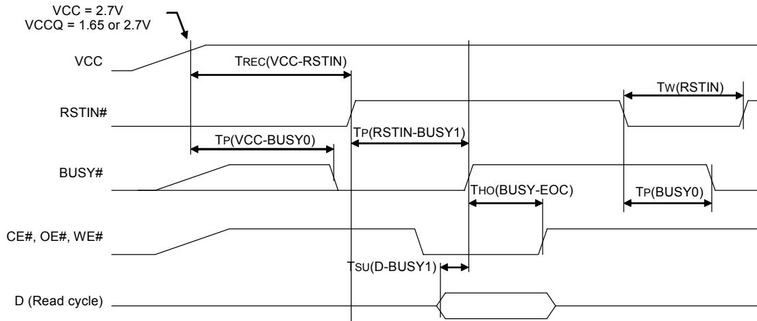
Figure 20: Reset Timing
