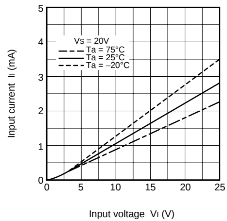
Input Characteristics
