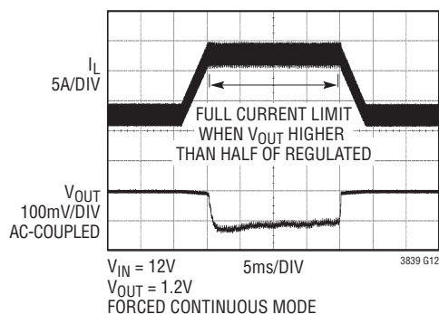
Overcurrent Protection
