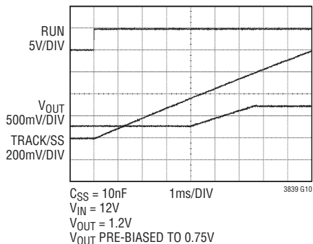
Soft Start-Up Into Pre-Biased Output
