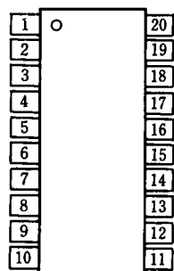
NJM2247AM / BM
