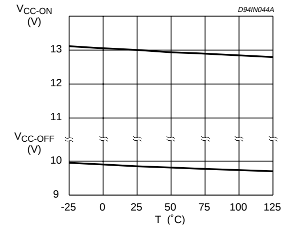
Figure 12. Undervoltage Lockout Threshold vs. Temperature
