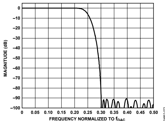
Figure 75. Interpolation Filter Response
