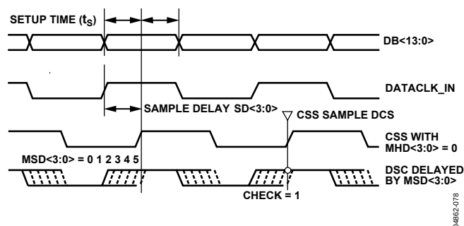
Figure 80. Setup Delay Measurement
