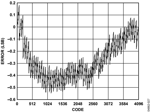
Figure 29. AD9735 INL, 25°C, 30 mA FS
