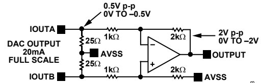
Figure 95. Differential Op Amp Output Circuit
