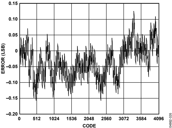
Figure 28. AD9735 INL, 25°C, 20 mA FS
