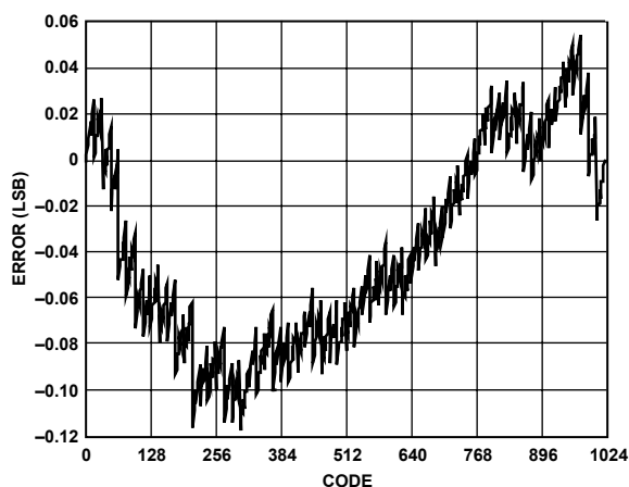
Figure 35. AD9734 INL, 25°C, 30 mA FS
