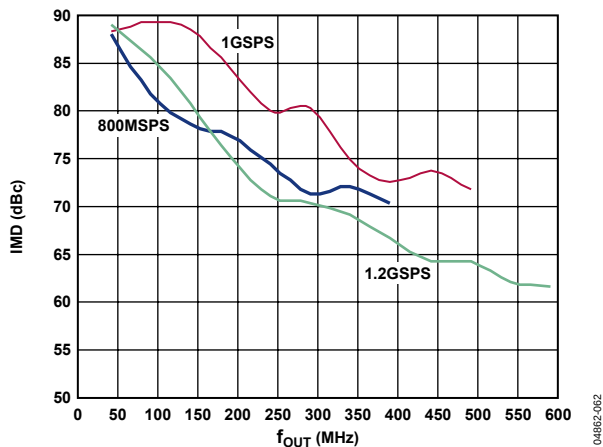
Figure 61. AD9735 IMD vs. f_{OUT} over f_{DAC} , 1.2 GSPS
