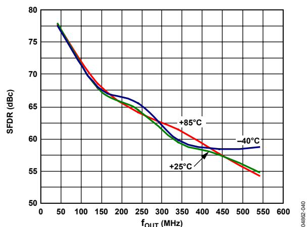
Figure 42. AD9736 SFDR vs. f_{OUT} over Temperature
