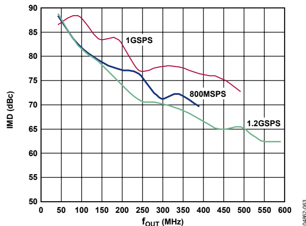
Figure 62. AD9734 IMD vs. f_{OUT} over f_{DAC} , 1.2 GSPS
