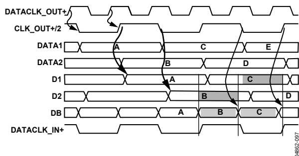
Figure 99. FPGA/ASIC Timing for Driving AD973x Digital Inputs, 2× Mode
