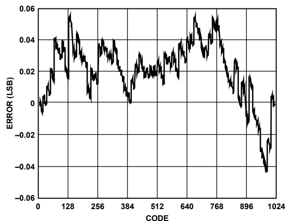
Figure 33. AD9734 INL, 25°C, 10 mA FS
