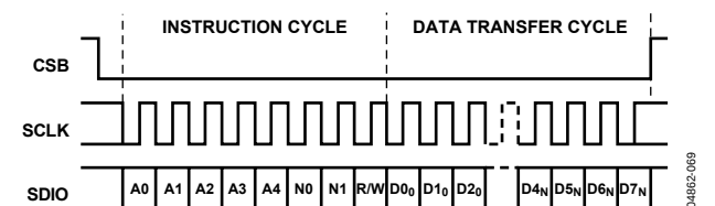
Figure 71. Serial Register Interface Timing, LSB-First Write
