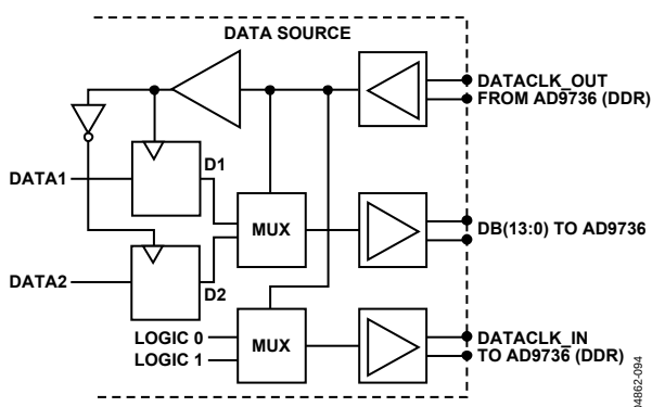
Figure 96. Recommended FPGA/ASIC Configuration for Driving AD9736 Digital Inputs, 1× Mode
