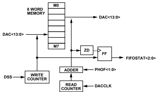
Figure 82. Sync Logic Block Diagram
