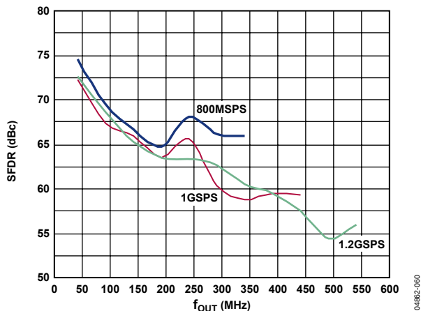
Figure 59. AD9735 SFDR vs. f_{OUT} over f_{DAC} , 1.2 GSPS
