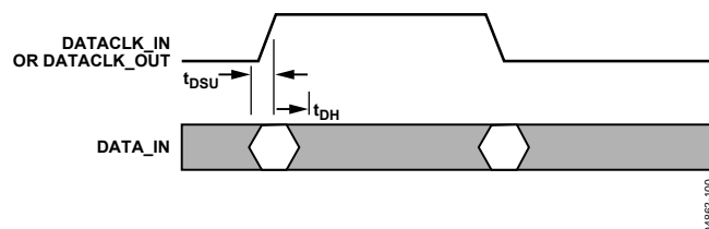
Figure 102. Standard Definitions for DATACLK_IN or DATACLK_OUT to Data Setup and Hold, SD = 0
