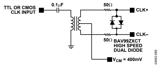
Figure 91. TTL or CMOS DACCLK Drive Circuit
