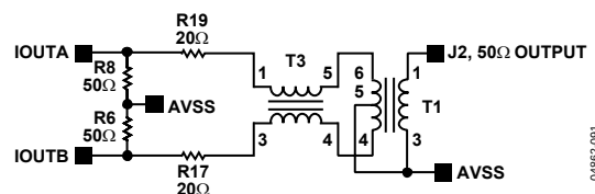
Figure 93. IF Signal Output Circuit
