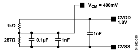
Figure 92. DACCLK V_{CM} Generator Circuit
