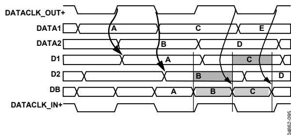
Figure 97. FPGA/ASIC Timing for Driving AD973x Digital Inputs, 1× Mode
