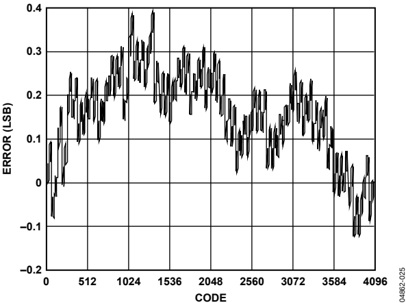
Figure 27. AD9735 INL, 25°C, 10 mA FS
