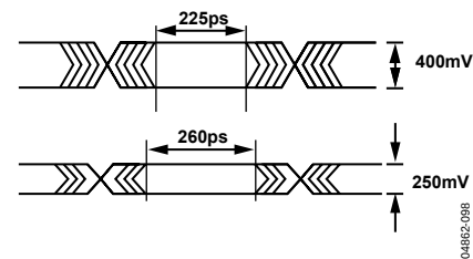
Figure 100. Typical Minimum Valid Data Time ( t_{MDE} ) vs. LVDS Swing
