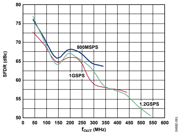
Figure 60. AD9734 SFDR vs. f_{OUT} over f_{DAC} , 1.2 GSPS
