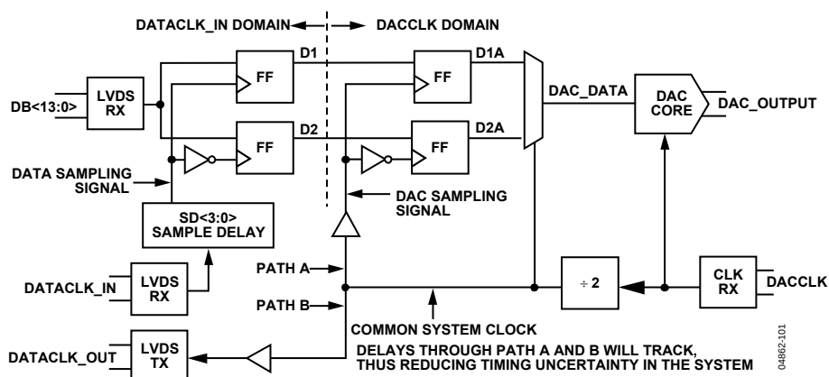
Figure 103. Simplified Internal Clock Routing
