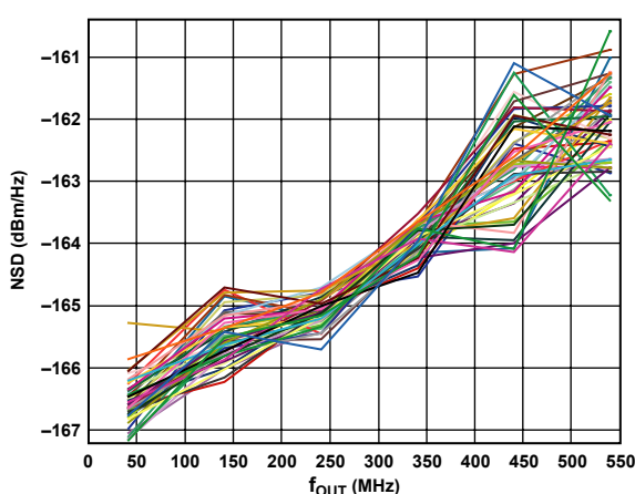
Figure 58. AD9736 8-Tone NSD vs. f_{OUT} over 50 Parts, 1.2 GSPS, 25°C
