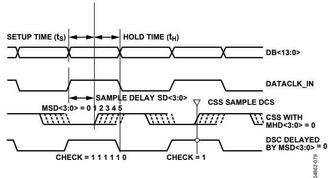
Figure 81. Hold Delay Measurement
