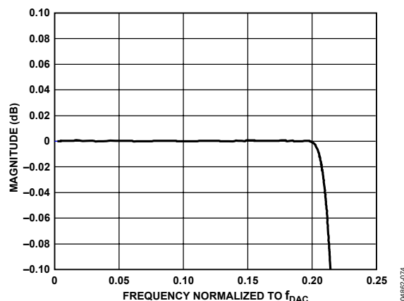
Figure 76. Interpolation Filter Pass-Band Flatness
