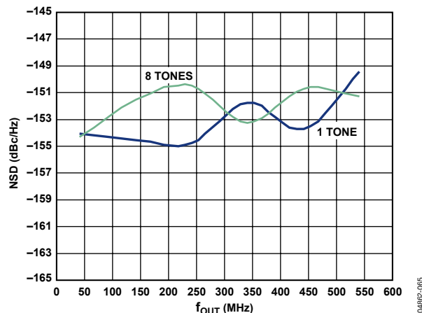
Figure 64. AD9734 NSD vs. f_{OUT} , 1.2 GSPS
