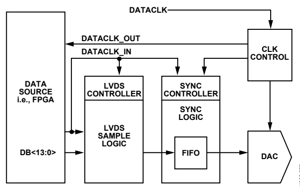
Figure 77. Data Controllers
