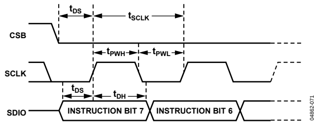
Figure 73. Timing Diagram for SPI Register Write
