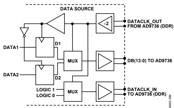
Figure 98. Recommended FPGA/ASIC Configuration for Driving AD9736 Digital Inputs, 2× Mode
