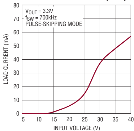
Minimum Load to Full Frequency
