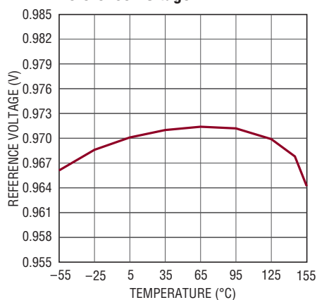
Reference Voltage
