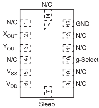
Figure 4. Pinout Description
