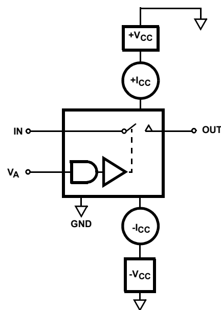
FIGURE 6. SUPPLY CURRENTS
