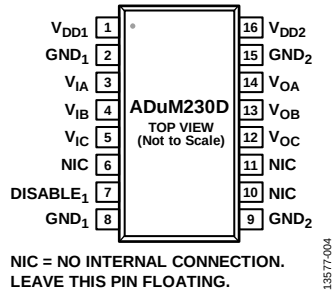
Figure 6. ADuM230D Pin Configuration
