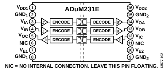
Figure 4. ADuM231E Functional Block Diagram
