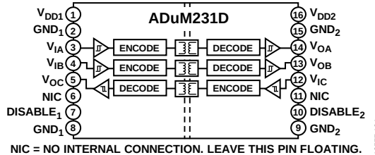
Figure 3. ADuM231D Functional Block Diagram
