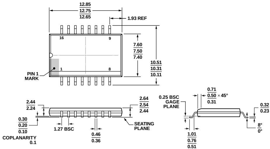
Figure 23. 16-Lead Standard Small Outline Package, with Increased Creepage [SOIC_IC] Wide Body (RI-16-2)
