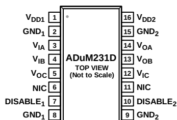
Figure 8. ADuM231D Pin Configuration
