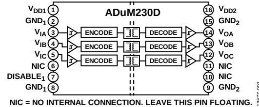
Figure 1. ADuM230D Functional Block Diagram
