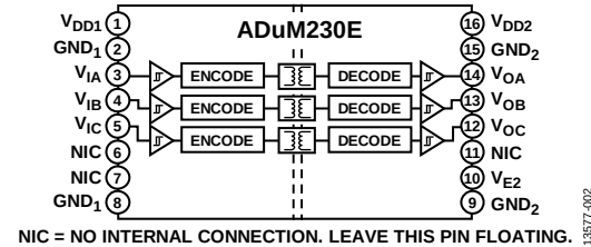
Figure 2. ADuM230E Functional Block Diagram
